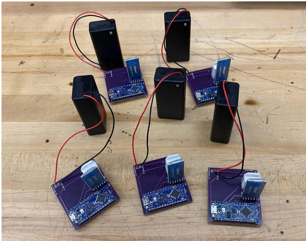
Fig. 2 The five sensor units on their PCBs
