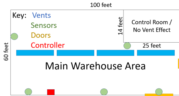
Fig. 11. Sensor Placement Diagram
