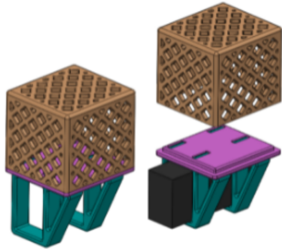
Fig. 3. Sensor Casing designed in Solidworks
