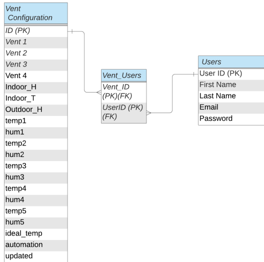
Fig. 7. Entity Relationship Diagram
