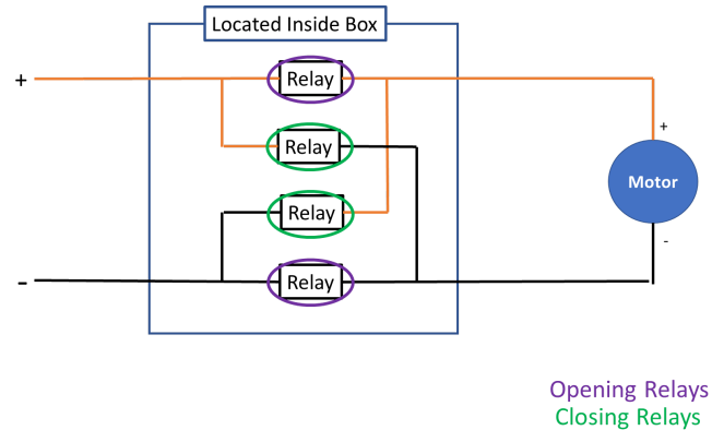
Fig. 4. Relays Wiring Diagram
